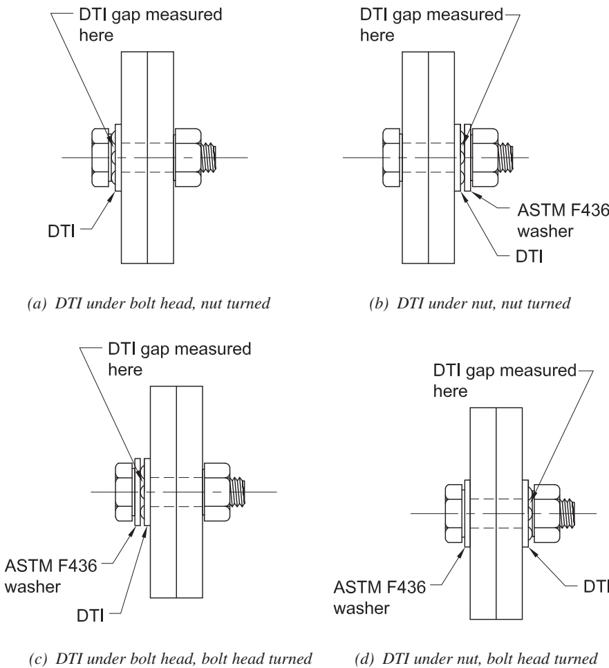
Fig. C-8.1. Proper use and orientation of ASTM F959 direct tension indicators.
